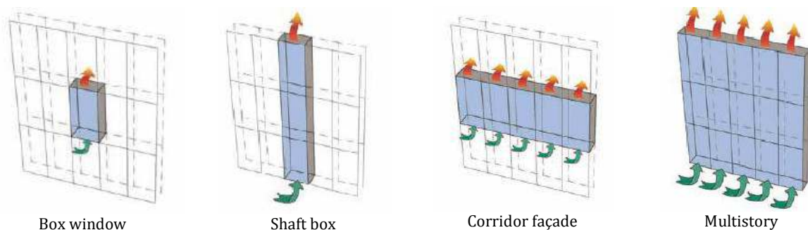
Gambar 2. Tipe DSF (Sumber: Tascon, 2008)
